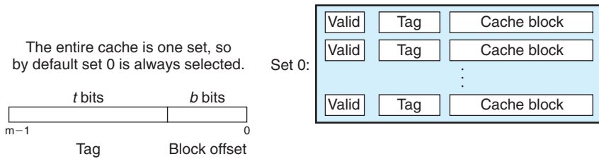
Figure 6.38 Set selection in a fully associative cache. Notice that there are no set index bits.
